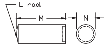
#602 Rocker Pin
