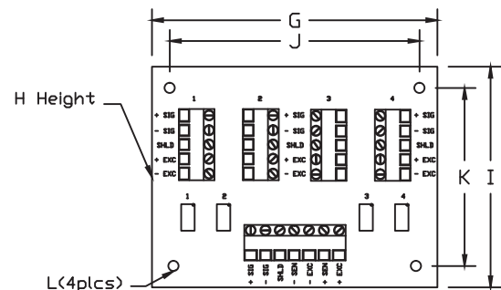
Summing Card
