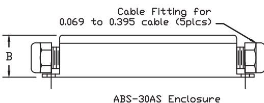
ABS-30AS Enclosure
