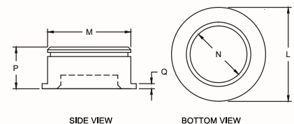
TOP PLATE #630 & #632
