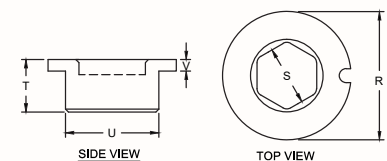
BOTTOM PLATE #631 & #633
