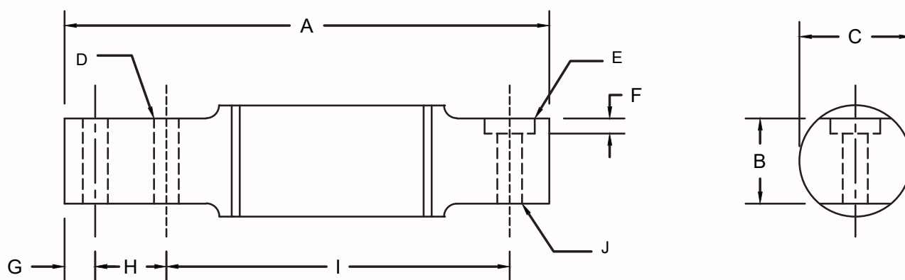
Main Dimensions and Accessories
